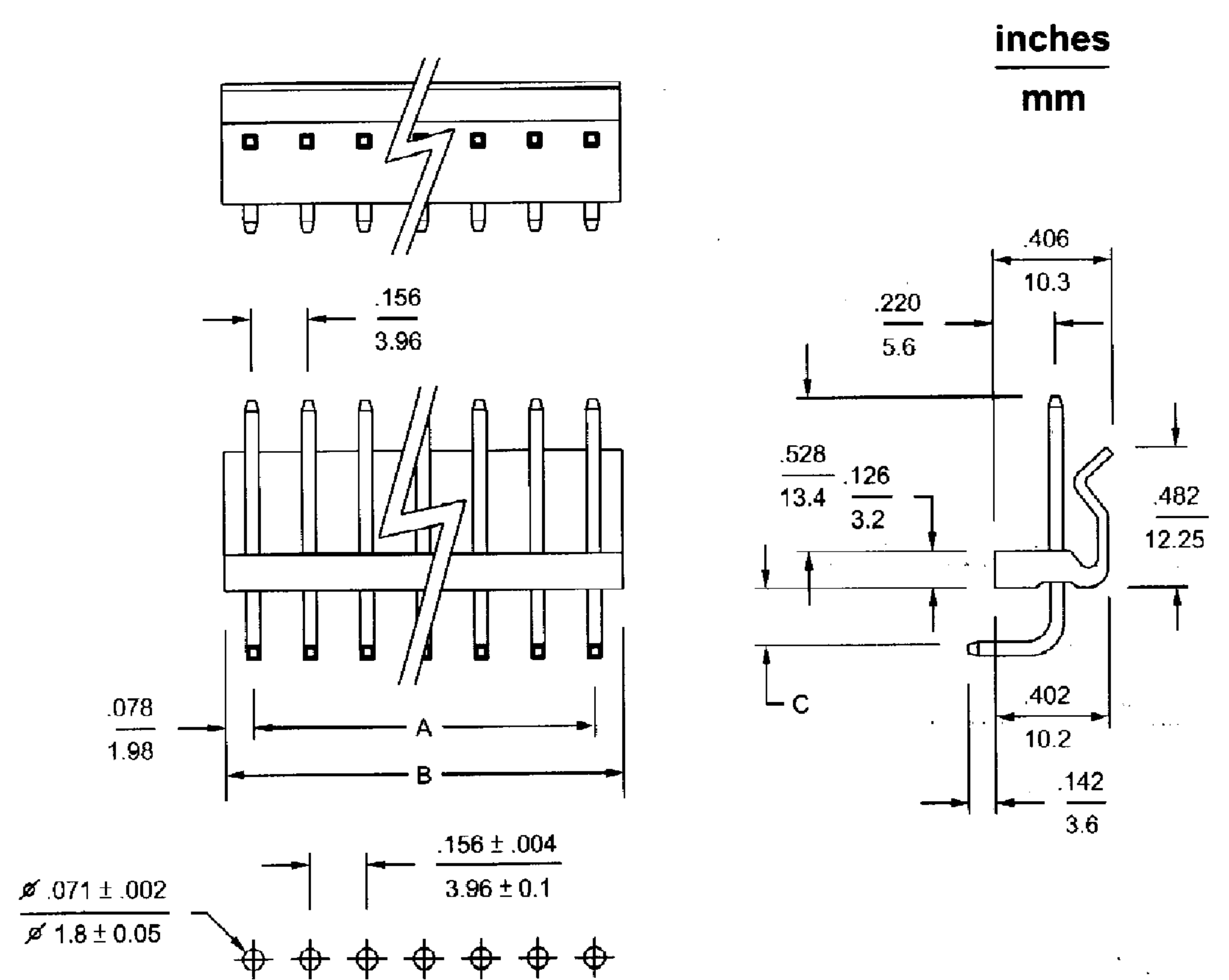
P. C. B. hole dimensions
