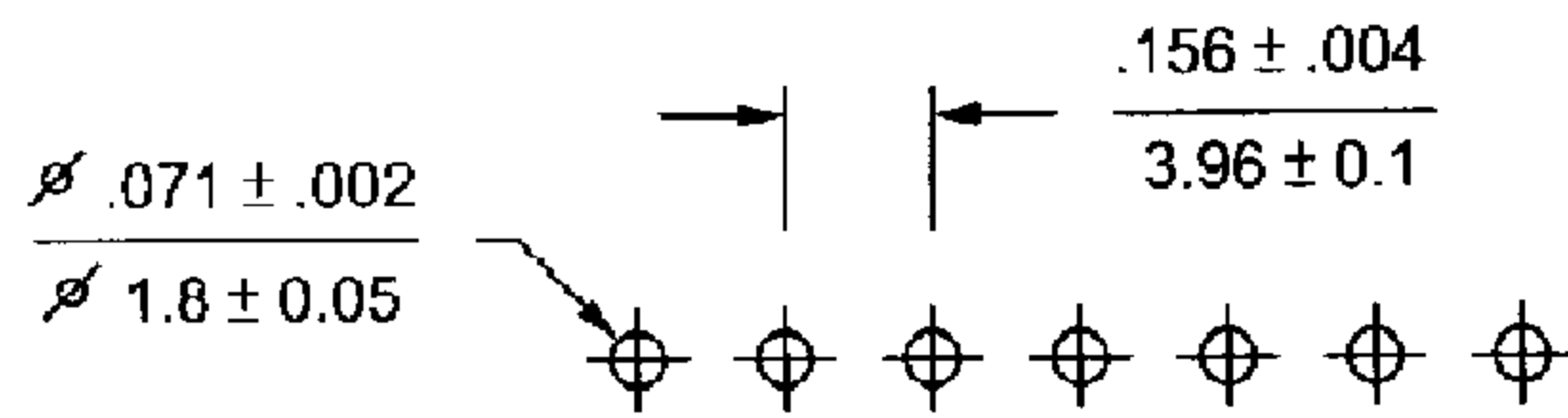
P. C. B. hole dimensions
