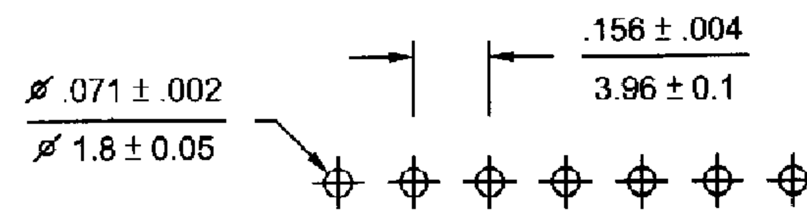
P. C. B. hole dimensions
