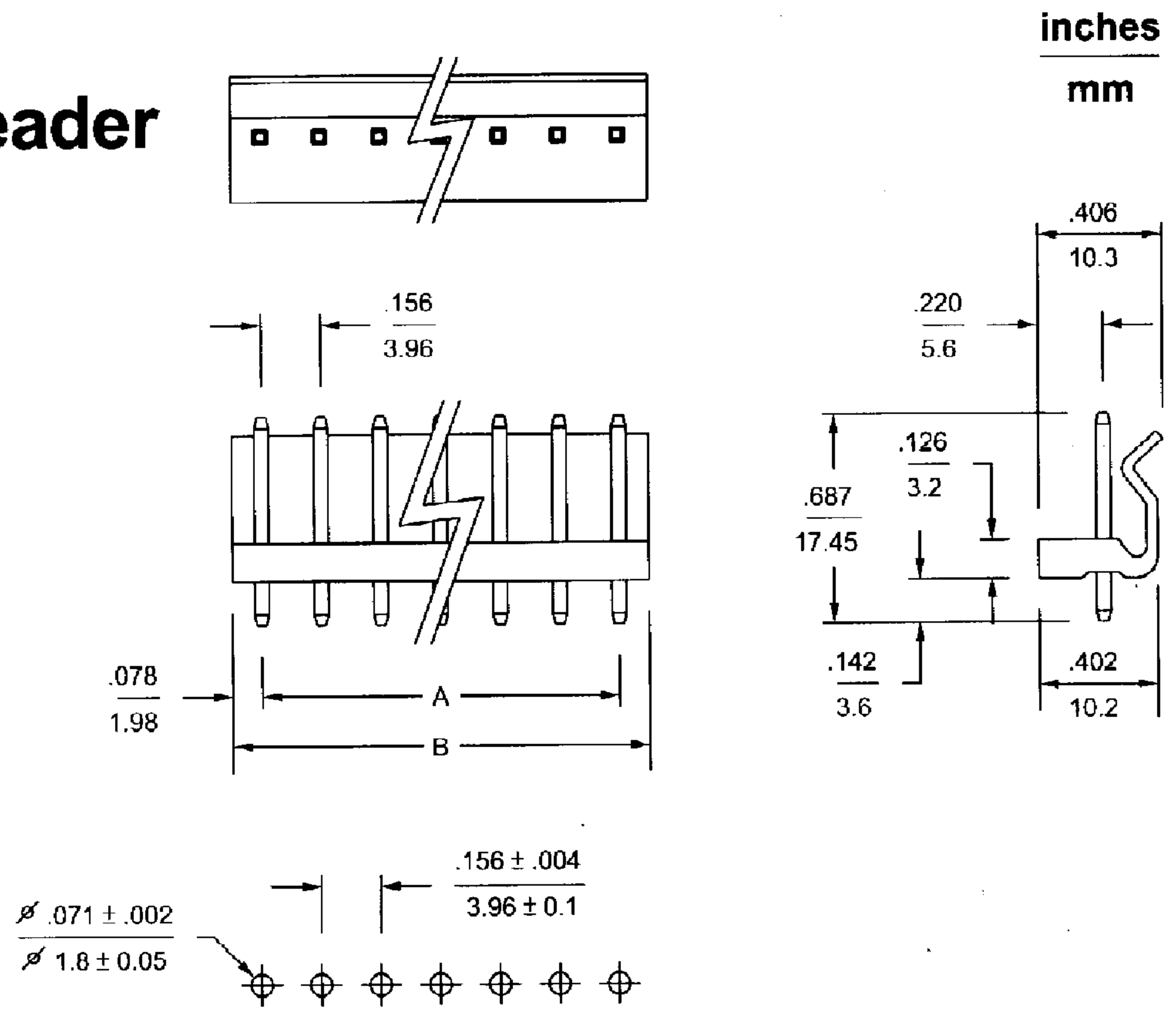
P. C. B. hole dimensions
