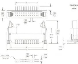
P. C. B. hole dimensions
