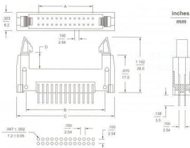
P. C. B. hole dimensions
