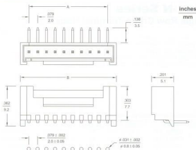
P. C. board hole dimensions
