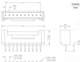
P. C. board hole dimensions
